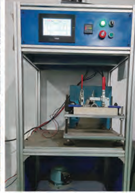
◆ Drill lifetime testing machine
